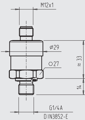
with M12 x 1 circular connector
